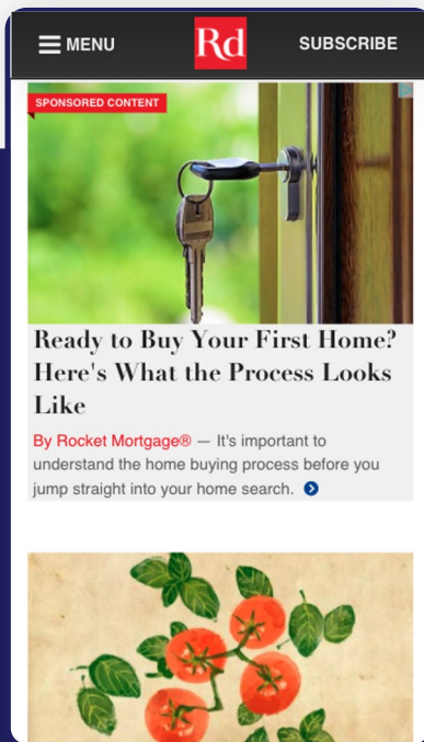
Native In-Feed
