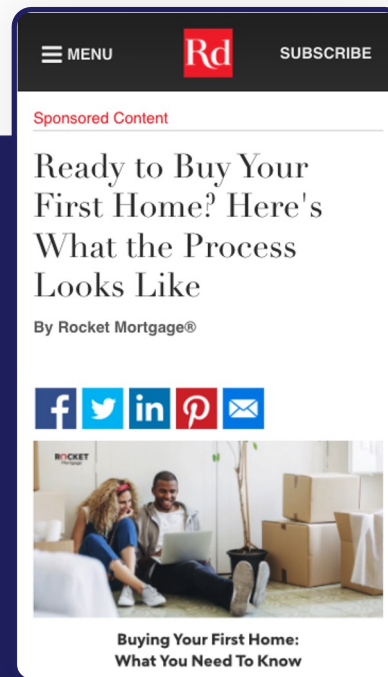
Native Article
